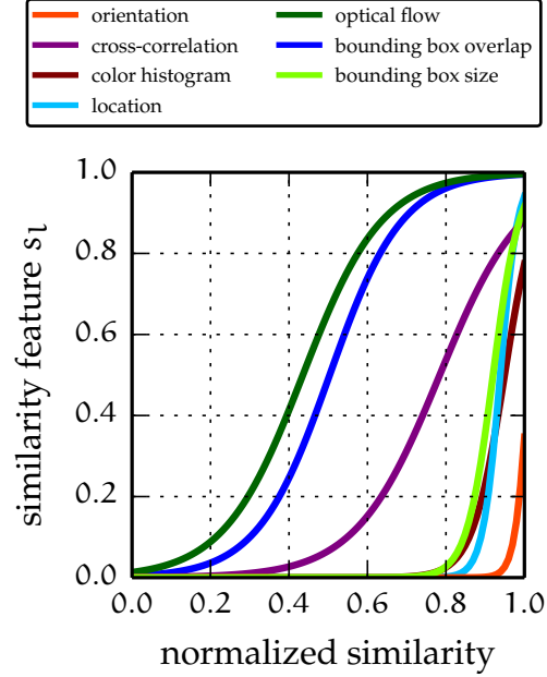
Figure 4: Similarity Features. Logistic functions learned that transform each raw feature l (e.g., bounding box IOU) into an association score s_l (similarity). We learn all logistic functions via logistic regression on the KITTI training set using the ground truth associations.
