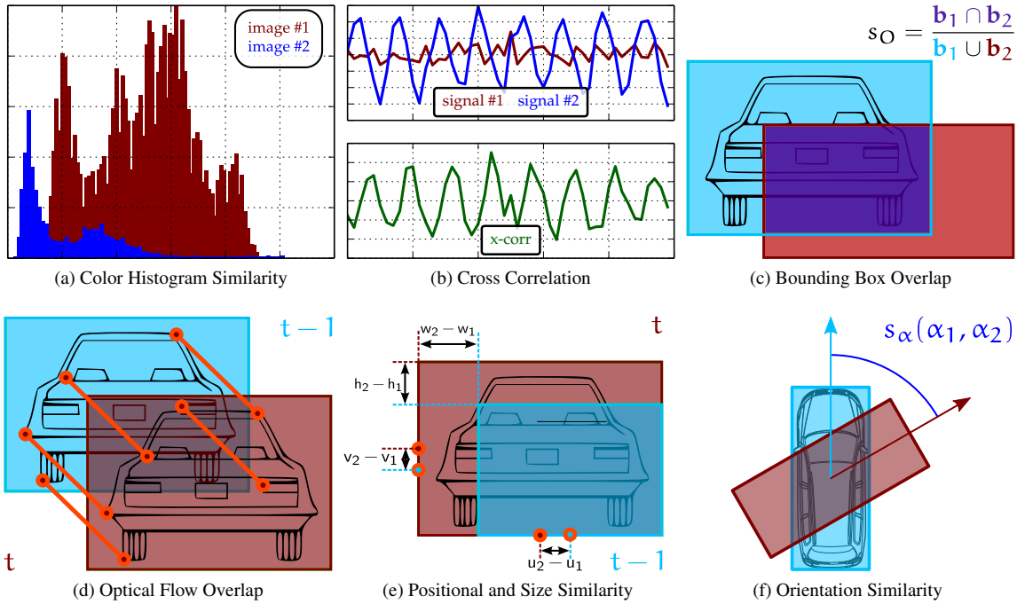
Figure 1: Association Features. Image-based ((a), (b)) and positional-based ((c), (d), (e), (f)) features used as input for association costs within the network flow formulation.
