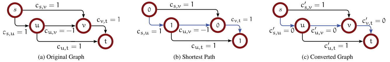
Figure 18: Cost Conversion Example. For the graph in (a) with negative costs, the shortest s-t path is computed (blue edges in (b)). Numbers in the nodes state the distance on the shortest path for this particular node. The graph is converted into a graph without negative costs according to Eq. 6. The resulting graph in (c) contains the arborescence \Gamma in blue which is identical with the shortest s-t path in this case.
