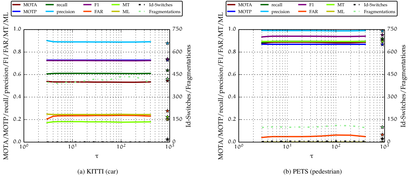
Figure 7: Performance for Different History Lengths. We evaluated the performance of mbodSSP for different values of its history length \tau on the whole KITTI training set and PETS S2.L1. Result for \tau \rightarrow \infty are given on the very right of the plot.
