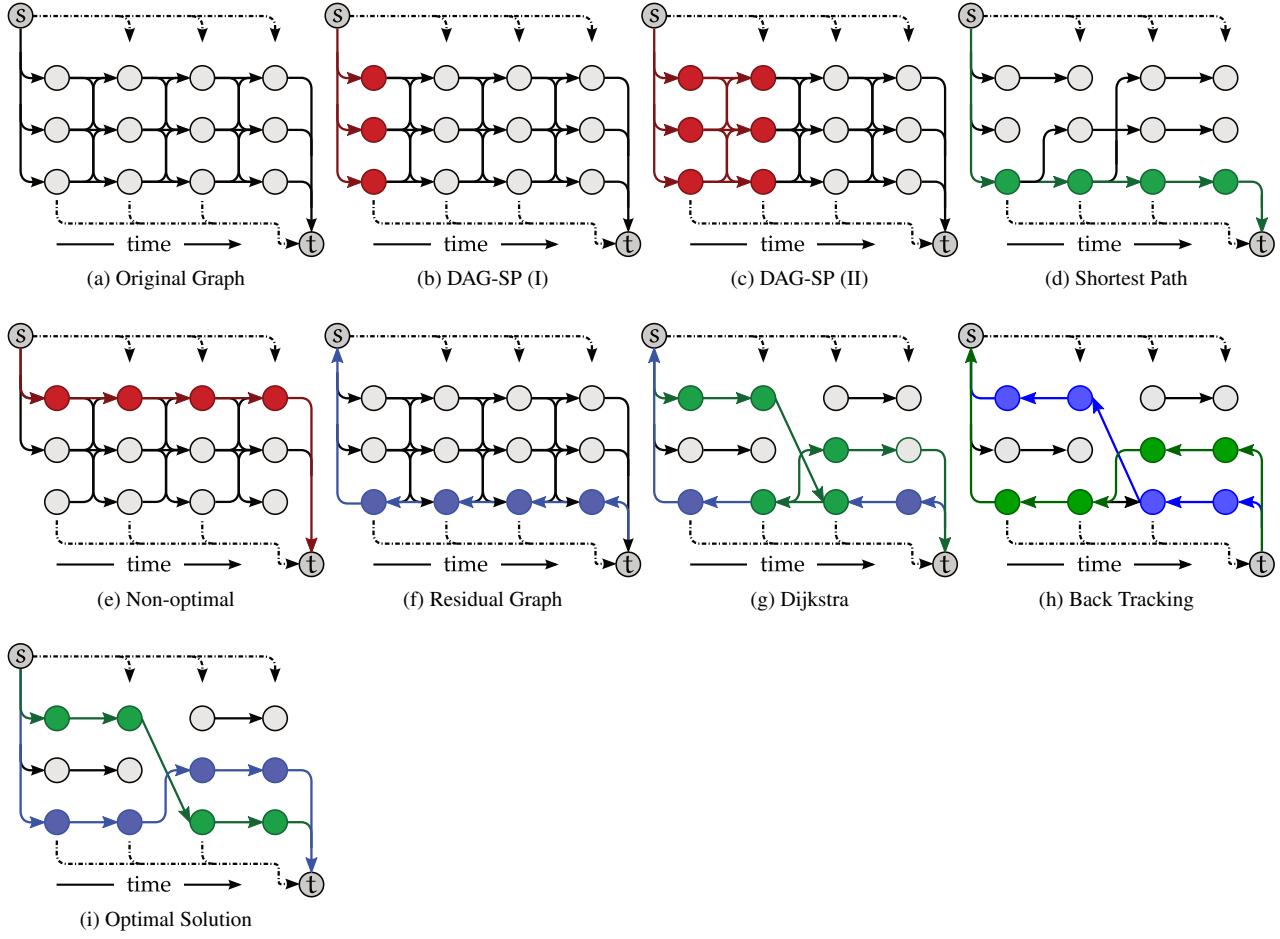
Figure 16: Illustration of the SSP Algorithm. The original problem is depicted in (a). Dynamic programming relaxes the red edges in (b) and (c) yielding the shortest path in the DAG, depicted in green in (d). Simply removing this path and re-running the algorithm violates optimality as shown in (e). Instead, a SSP strategy on the residual graph (f) allows for finding the optimal solution (g+h). Backward pointing edges in the residual graph (h) encode trajectories for the original problem (i).
