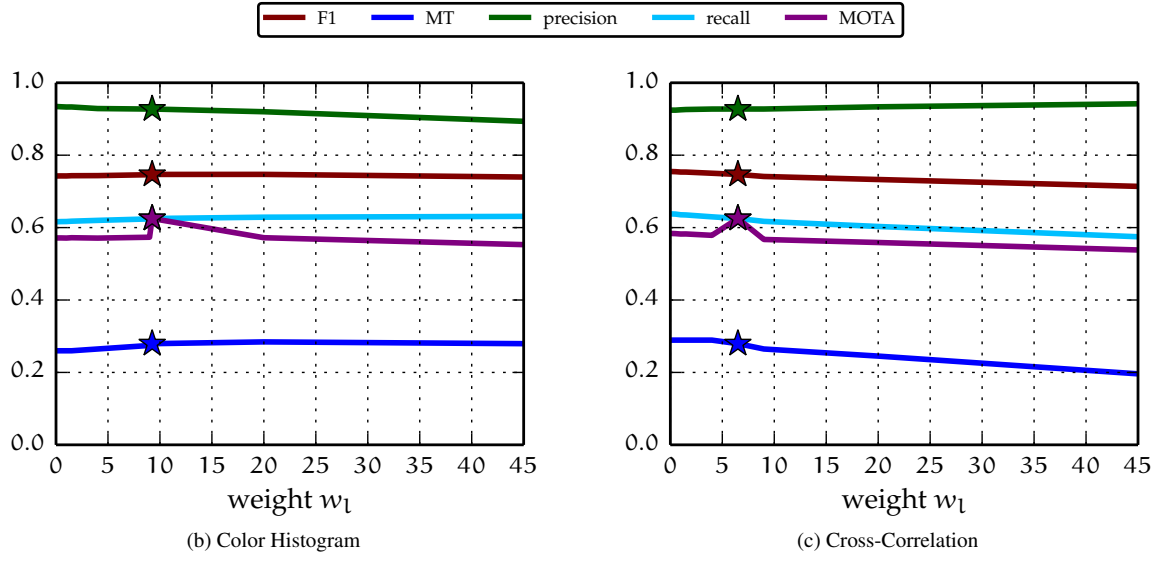
Figure 6: Robustness of Appearance-based Features against Variation of Parameters. This figure shows the performance dSSP for different weight values on the KITTI training set. While varying one parameter, all other parameters are kept fixed (c.f. Table 1).
