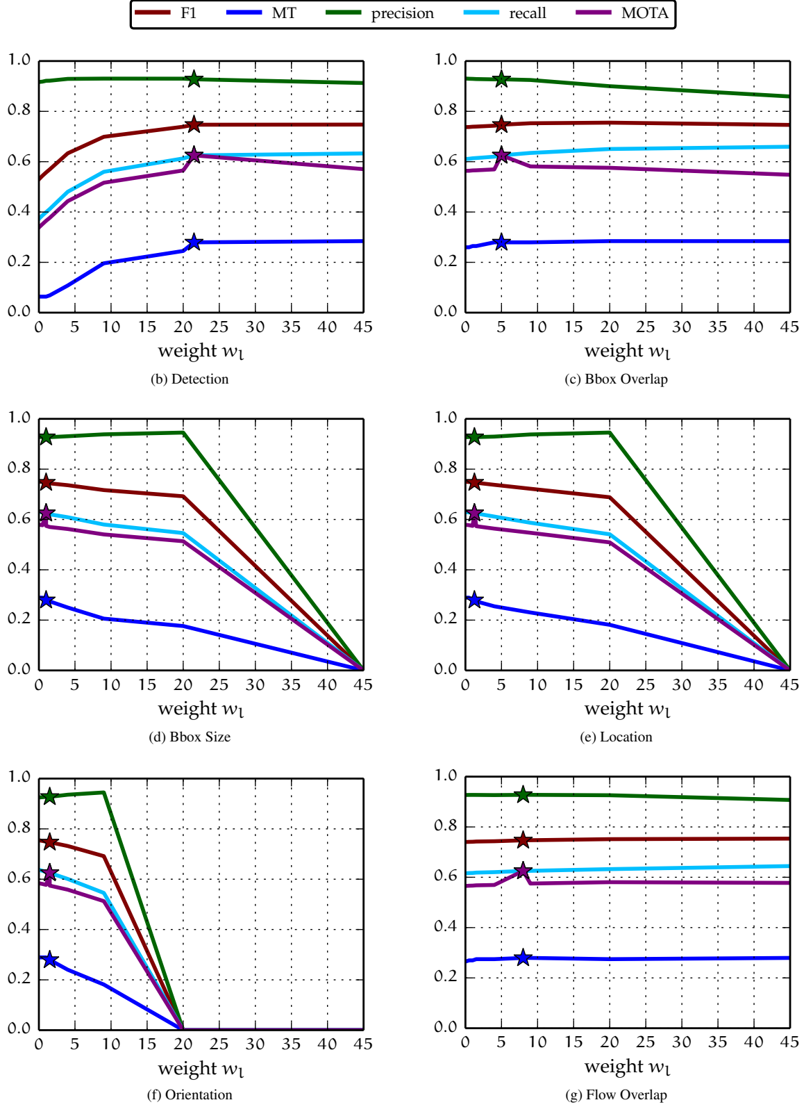
Figure 5: Robustness of Detection and Positional Features against Variation of Parameters. This figure shows the performance for different weight values on the KITTI training set using dSSP. While varying one parameter, all other parameters are kept fixed (c.f. Table 1).
