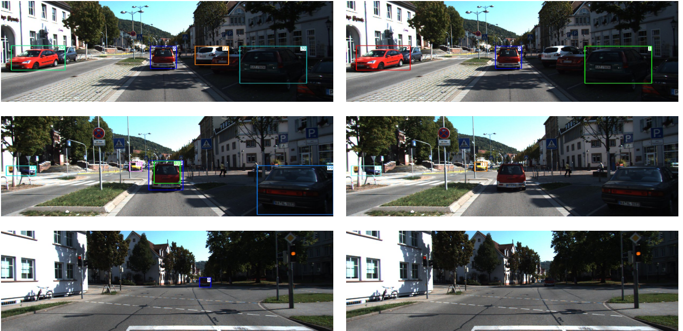
Figure 11: Qualitative Results for the Optimal (left) and our Approximate Solution (right). Changes in illumination and resulting ambiguous detections (middle) may lead the approximate solution to terminate a track due to missing future evidence. In contrast, the optimal solution tracks the preceding car for 37.2s.
