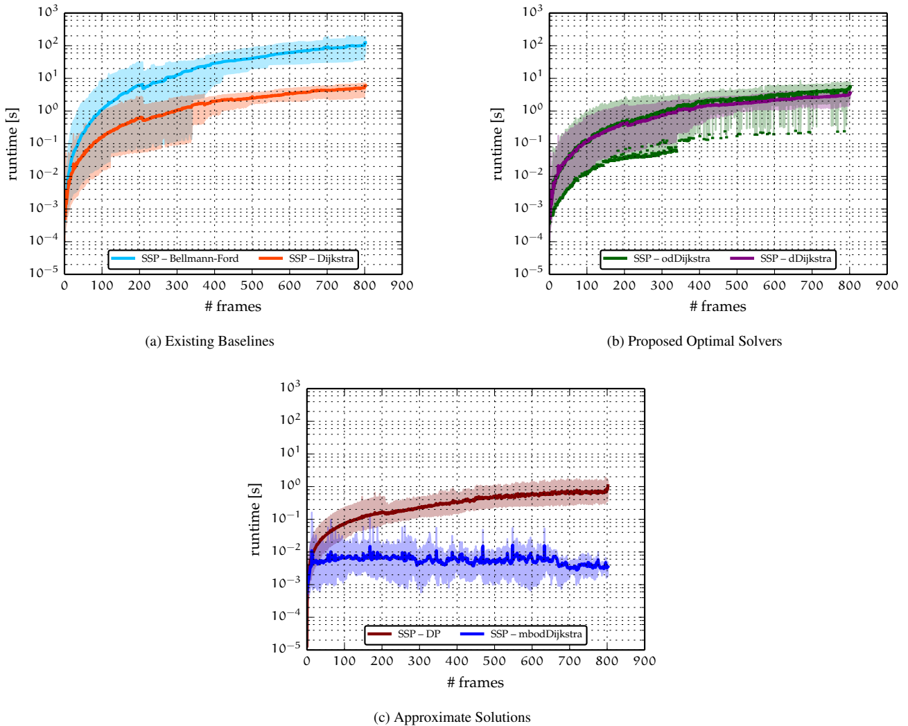
Figure 2: Comparing Run Time: Batch solvers are shown as a function of the sequence length in the first two figures. As shown in the last figure, our approach outperforms significantly [12], named SSP-DP in terms of runtime. We use a window size of \tau = 10 for mbodSSP and evaluate all methods on a the original network without pruning any edges.
